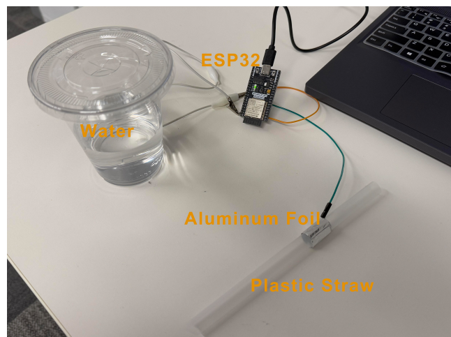
Figure 2: Hardware Design
